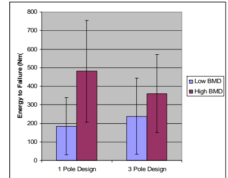
Figure 4- Chart showing energy to failure at high and low bone mineral density subgroups.
